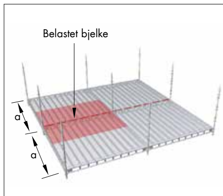
Utbredt stillase
